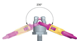
Pic. 2: Pivoting area of PP-S/PP-B/PP-VIP
