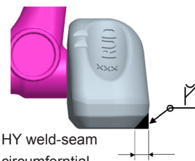
Picture 3: HY-weld seam
