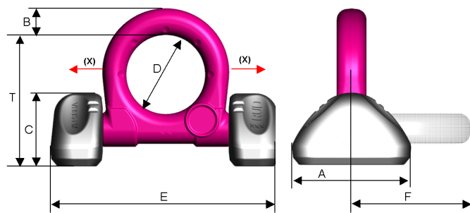
Picture 2: Dimensioning
